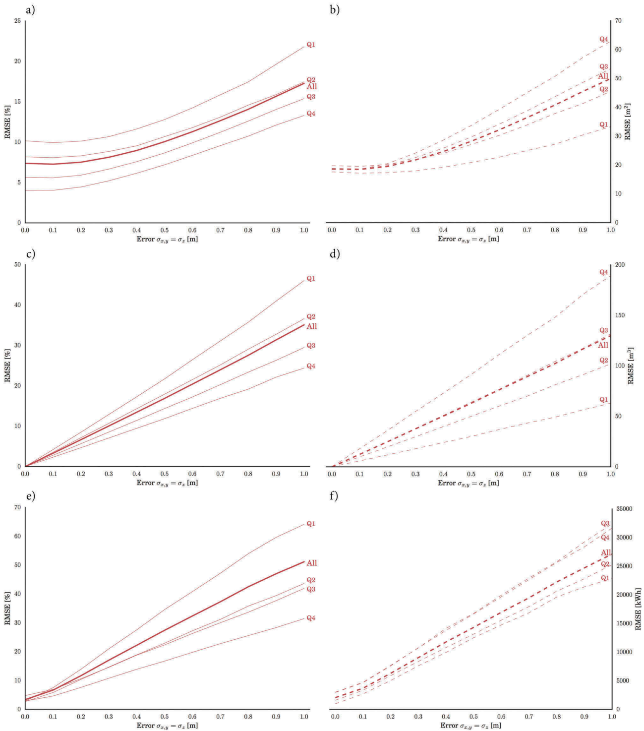
Figure 8. Dissecting the combined errors: building size influences the results. The plots on the left side show the errors in percentages, while the plots on the right express the errors in the units of measurements.
